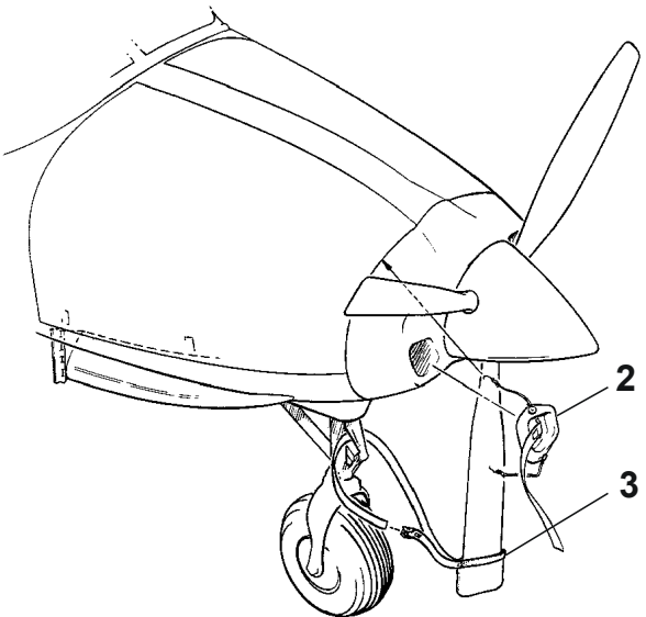
AIRPLANES 20800001 THRU 20800127 AND 208B0001 THRU 208B0054
