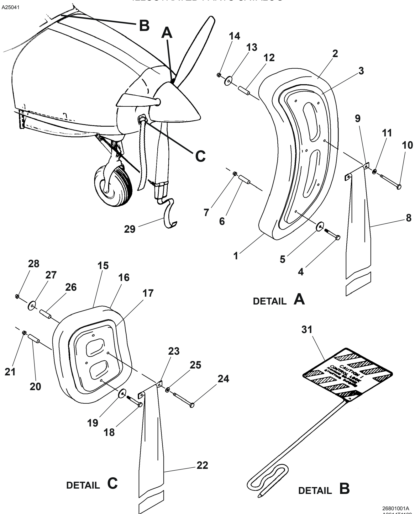
PARKING AND STORAGE EQUIPMENT Figure 02. (Sheet 1)
